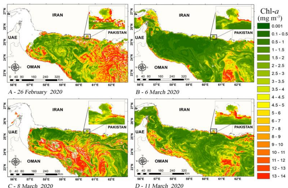
Figure 2: Chl- a change under the influence of N. scintillans in \text{mg m}^{-3} in the Oman Sea -Modis sensor.
