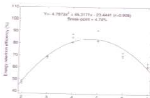
Figure 5: Second-order polynomial relationship between energy retention efficiency (ERE) and feeding levels for rainbow trout, Oncorhynchus mykiss fingerlings fed with experimental diets for 10 weeks ( n =mean of 3 replicates).
