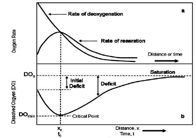
Figure 1: (a) Deoxygenation and reaeration responses to the organic material, and (b) the DO sag curve, which is characteristic of change of DO concentration in a river after the introduction of organic material.
