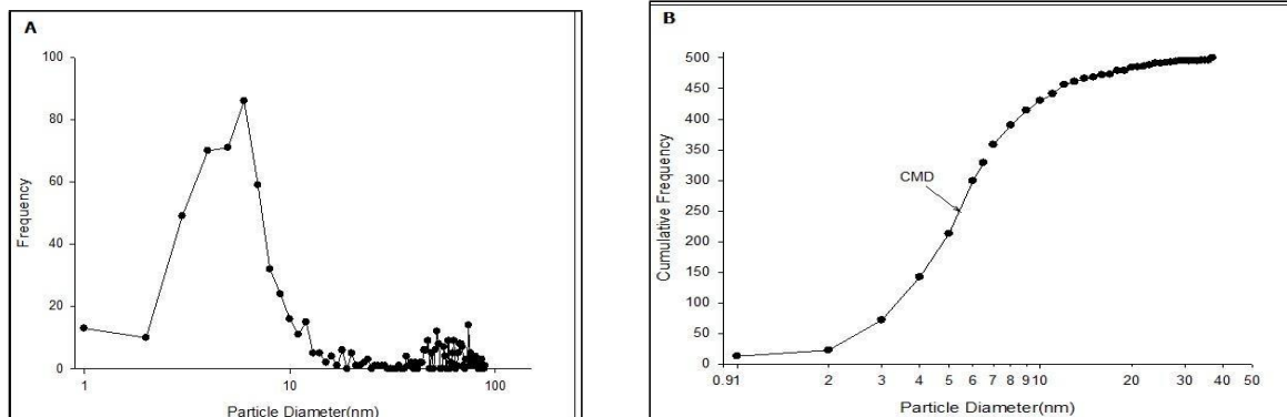
Figure 3: Size distribution of silver nanoparticles in undiluted suspension (4000 mg/L) based on transmission electron microscope (TEM) data. A: Number Frequency and B: Cumulative Frequency (CMD: Cumulative median diameter).
