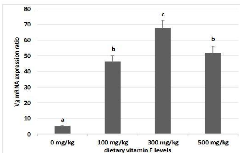
Figure 1: Vg mRNA expression ratio in the hepatopancreas of female L. vannamei fed with four experimental diets. The mean expression ratio±standard error of mean (SEM) (n=3) in the different groups are shown, with treatment at the x axis and expression ratio at the y axis. Statistical significance is indicated with different letters ( p<0.05 ).
