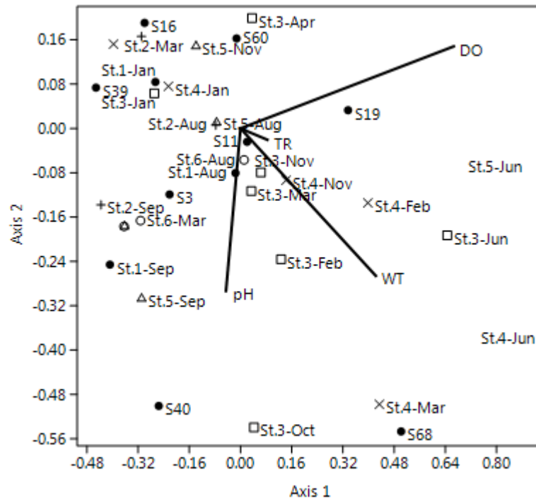
Figure 11: Canonical correspondence analysis (CCA) of fish abundance and hydrological parameters of Karatoya Fish Sanctuary.
