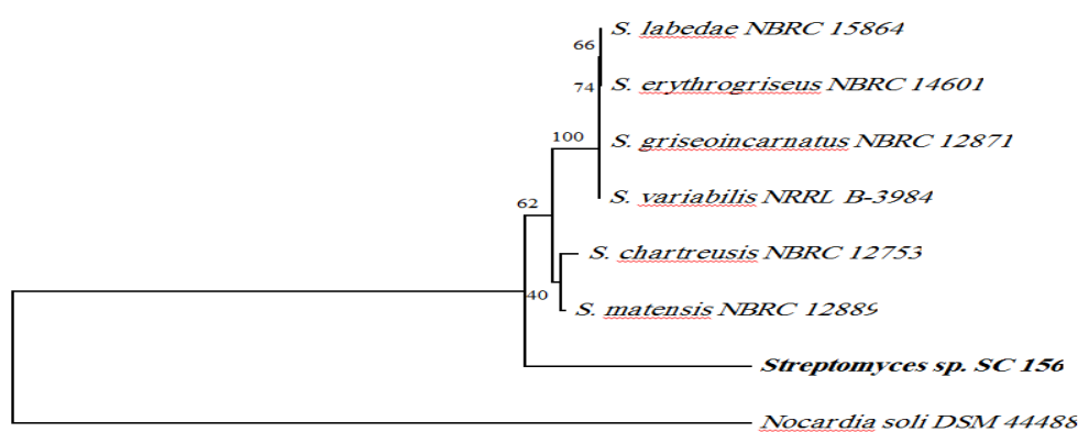
Figure 6: Phylogenetic tree based on 16S rRNA gene sequence analysis, reconstructed from evolutionary distances by using the neighbor-joining method, showing the phylogenetic position of potent strains and the most closely related strains. N. soli was used as an out-group. Bootstrap values are indicated at the relevant branching points. Numbers of branch node are bootstrap value based on 1000 resampling. Bar: 0.01 substitutions per nucleotide position.
