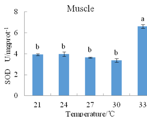
Figure 4: The effects of temperature on the immune enzymes activities in the hepatopancreas (a, c) and muscle (b, d) of Fenneropenaeus merguensis .
