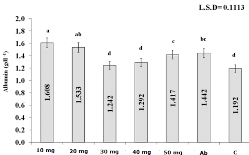
Figure 4: The effect of different concentrations of Excoecaria agallocha on albumin levels ( \text{gdL}^{-1} ). Columns with different letters are considered a significant difference ( p < 0.05 ). Ab-: Antibiotic group C-: Control group
