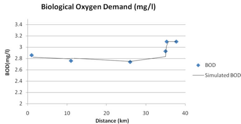
Figure 3: Model calibration for ultimate biological oxygen demand
