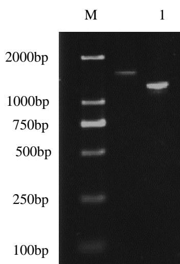
Figure 2: The electrophoresis result of PCR amplification of 16S rRNA (Lane 1) and gyrB gene (Lane 2) from the strain KC-2. M is DL2000 DNA Marker.
