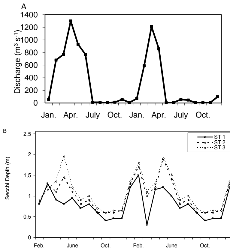
Figure 4. A: Monthly average of water flow (m 3 s -1 ) from Simav Stream to Çaygören Reservoir from January 2007 to December 2008; B: The variations in the Secchi disk depth (m) in the Çaygören Reservoir.
