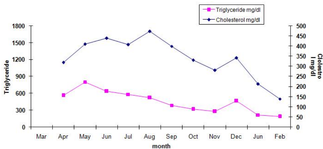
Figure 5: Changes in Triglyceride and cholesterol levels in female grey mullet ( M. cephalous ) in different months
