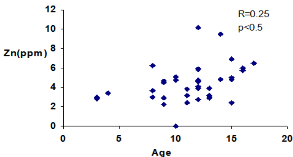
Figure 4: Concentration of Zn in muscles samples of A. stellatus in different ages (Dec.2007-June.2008)
