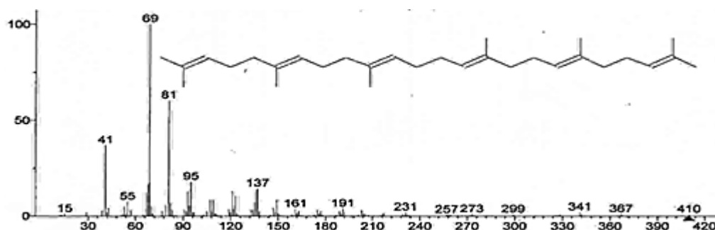
Figure 2: Mass spectrum of the squalene, corresponding to the major peak in the GC.
