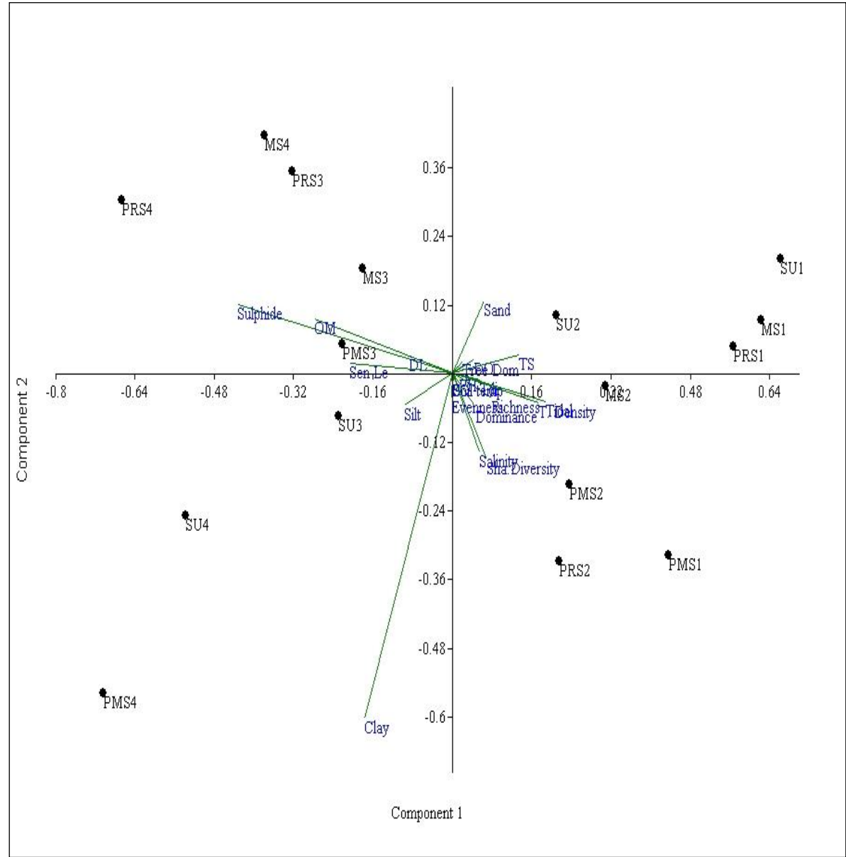
MS1monsoon station 1, MS2 monsoon station 2, MS3 monsoon station 3, MS4 monsoon station 4, PMS1 post-monsoon station1, PMS2 post-monsoon station 2, PMS3 post-monsoon station 3, PMS4 post-monsoon station 4, SU1 Summer station 1, SU2 Summer station 2, SU3 Summer station 3, SU4 Summer station 4, PRS1 pre-monsoon station 1, PRS2 pre-monsoon station 2, PRS3 pre-monsoon station 3, PRS4 pre-monsoon station 4
