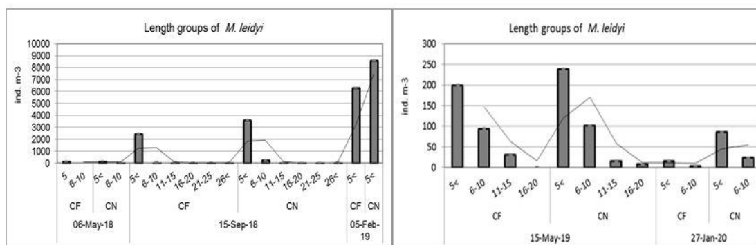
Figure 5: M. leidy length groups at near stations (CN) and far from cage fish farming site (CF), 2018-2020.
