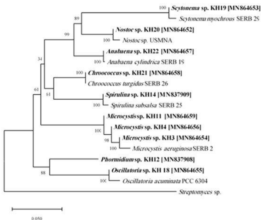
Figure 7: Phylogenetic tree based on 16S rRNA gene sequence analysis, reconstructed from evolutionary distances by using the neighbor-joining method, showing the phylogenetic position of the isolated cyanobacterial strains (Bold font) and type strain in NCBI GenBank. Bootstrap values are indicated at the relevant branching points. Numbers of branch node are bootstrap values based on 1000 resampling. Bar 0.02 substitutions per nucleotide position. Streptomyces sp. was used as an out-group.
