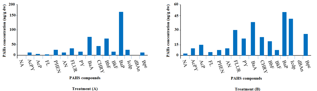
Figure 5: PAHs compounds in APC station during the cold (A) and warm (B) seasons.
