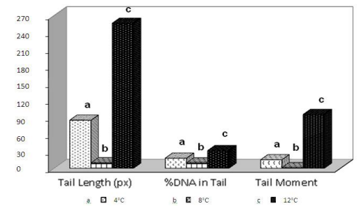
Figure 2: Caspian trout DNA damage description by total means for TL, DT & TM variables of Comet assay, 3 separated groups indicated by a (4°C), b (8°C), c (12°C).
