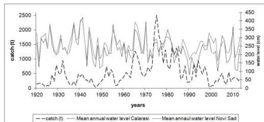
Figure 2: Fluctuations of mean annual Danube water level at Novi Sad and Călărași stations and fluctuation of Alosa immaculata annual catch.
