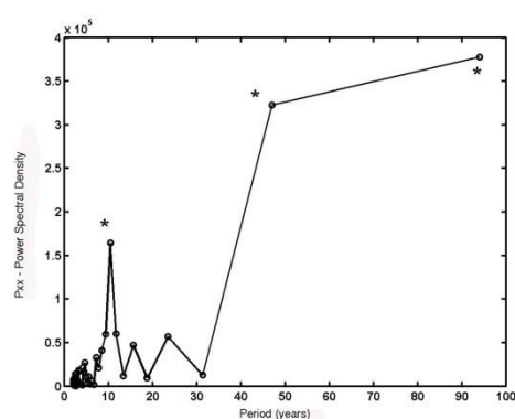
Figure 4: Spectral density of the catch of Alosa immaculata . (*) significant amplitudes.
