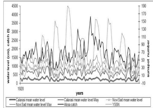
Figure 3: Relationship between mean annual Danube water levels and water levels in May at both stations, Novi Sad and Călărași, and catch of Alosa immaculata and solar activity.
