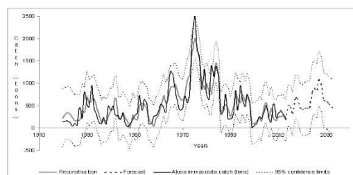
Figure 5: Reconstruction (1920-2013) and forecast (2014 - 2033) of the mean annual catch of Alosa immaculata from the Danube River in Romania, obtained by summing cyclical and stochastic components.
