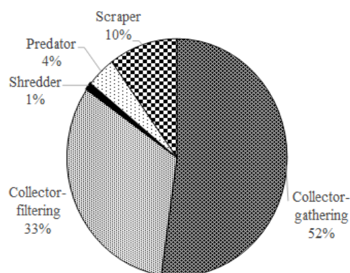
Figure 3: Overall percentage of the functional feeding groups in the sampling stations.
