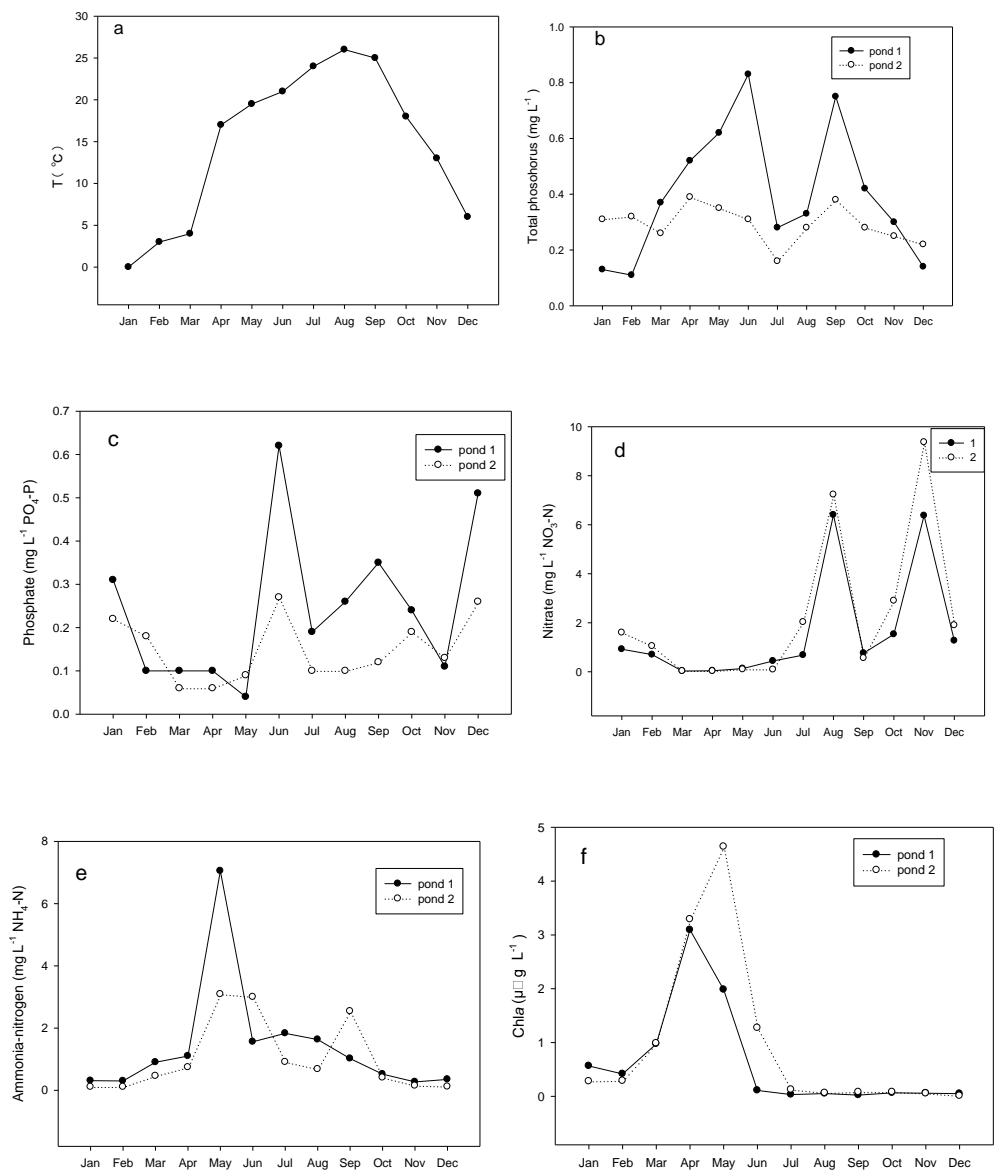
Figure 1: Seasonal variations in temperature (a), total phosphorus (b), phosphate (c), nitrate-nitrite (d), ammonium (e), and chlorophyll a (f) from January to December 2011 for culture of Carassius auratus gibelio in two ponds.
