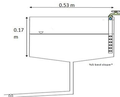
Figure 3: Typical scheme of laboratory 'Cornell-type' dual-drain tank.
