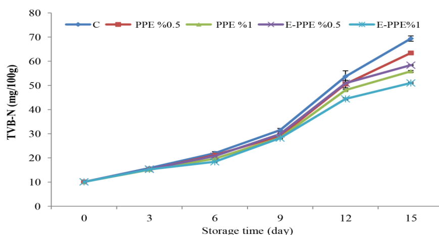
Figure 1: Changes in total volatile base nitrogen ( \text{mg N}_2 \text{ 100g}^{-1} ) value of silver carp fillets during storage.
