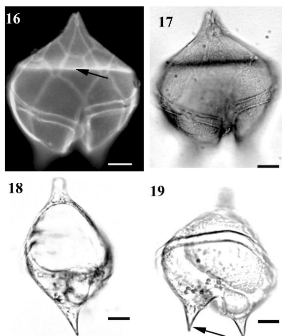
Figures 16-19: Protoperidinium claudicans . All scale bars=10µm
