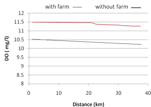
Figure 4: Simulation results for DO (mg/l)
