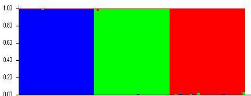
Figure 3: Clustering assignment of the three populations provided by STRUCTURE analyses
