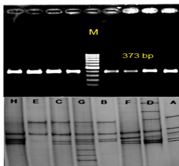
Figure 1: PCR product of Exon 4, Intron 4, and Exon 5 of GH-I gene (left) and banding patterns observed for GH-I gene (right) in common carp; M: molecular weight marker (mi-E8200s, 50 \mu g).
