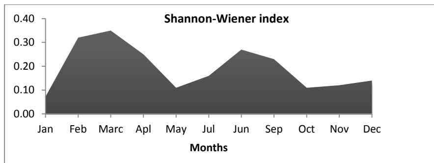
Figure 4: The variation of Shannon-Weiener diversity connects to months.
