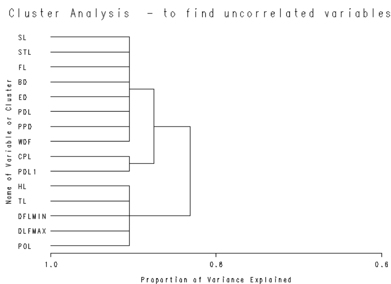
Figure 2: Cluster dendrogram for Nemipterus japonicus using morphometric and meristic variables (Chennai and Kochi, 2013).
