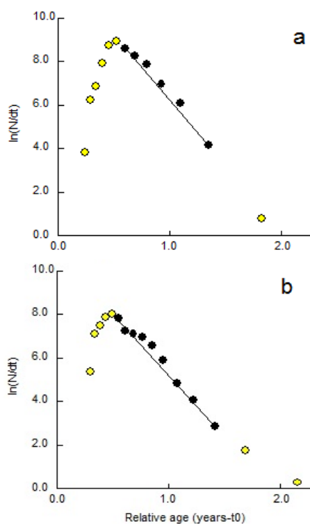
Figure 5: Length converted catch curve of Penaeus merguensis (a: male; b: female).
