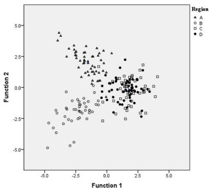
Figure 2: Plot of canonical variables (Function 1 and 2) of morphometric variables of Uroteuthis duvaucelii in the Persian Gulf and Oman Sea.
