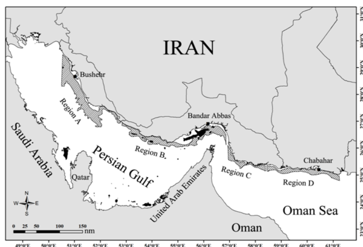
Figure 1: Sample locations (shaded areas) of the Indian squid ( Uroteuthis duvaucelii ) in the Persian Gulf and Oman Sea.
