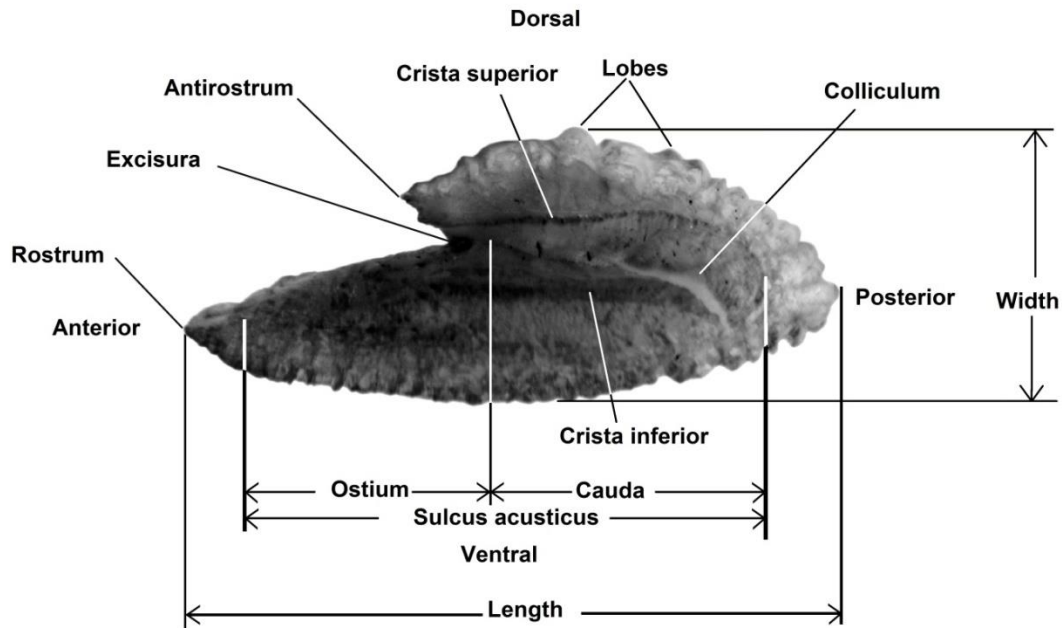
Figure 2: Proximal surface of sagittal otolith of Carangoides chrysophrys .
