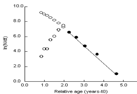
Figure 4: Length-converted catch curve for Liza klunzingeri in Iranian waters Note: only black dots have been considered for computation of total mortality.
