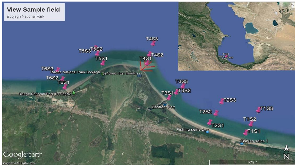
Figure 1: Study area and sites of sampling, Boojagh Marine National Park (6 transect; 18 sampling stations).
