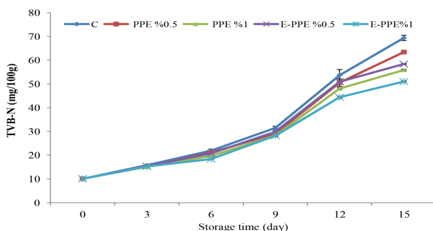
Figure 1: Changes in total volatile base nitrogen ( \text{mg N}_2 100\text{g}^{-1} ) value of silver carp fillets during storage.
